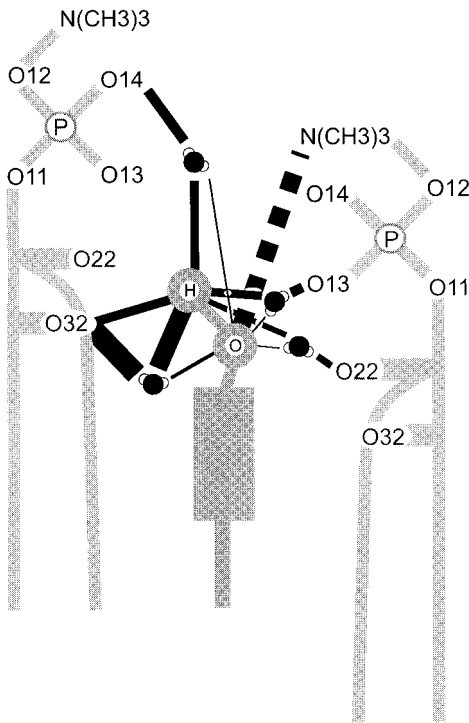
FIGURE 10 Partners with which the hydroxyl group of Chol is linked to a DMPC molecule. A solid line indicates a direct H bond, a dashed line indicates a charge pair, and a water molecule indicates a water bridge. The thickness of the line represents the probability of the link. Light gray indicates DMPC molecules; dark gray indicates a Chol molecule.
