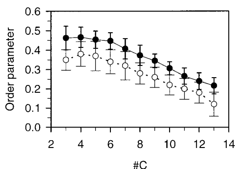
FIGURE 4 The molecular order parameter ( S_{\text{mol}} ) profiles calculated for the DMPC-Chol membrane (●) and for the pure DMPC membrane (○) at 310 K (averaged over \beta - and \gamma -chains, and over 2000 ps). Error bars are standard deviations.
